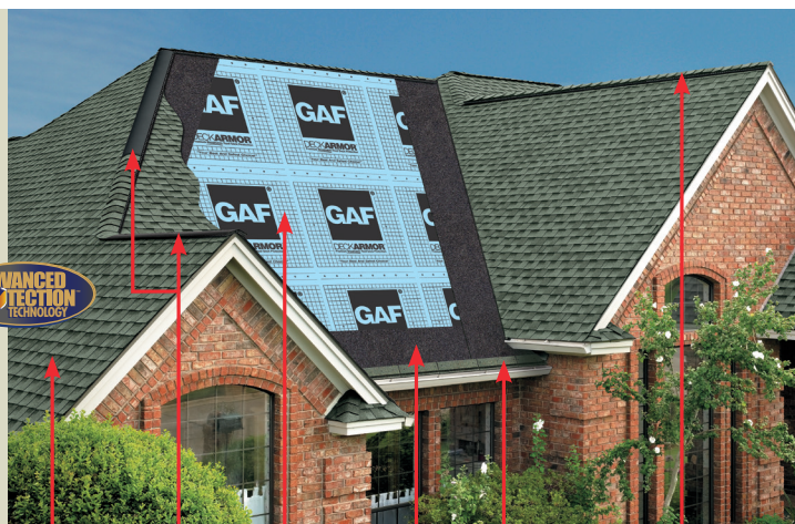
LIFETIME SHINGLES COBRA ATTIC VENTILATION ROOF DECK PROTECTION LEAK BARRIER STARTER STRIP SHINGLES RIDGE CAP SHINGLES
